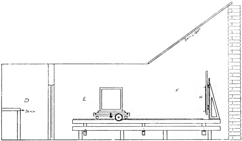
FIG. 11a.—Section of a Studio for North Light. D is the dark room, E the camera, F the stand, H the easel.
